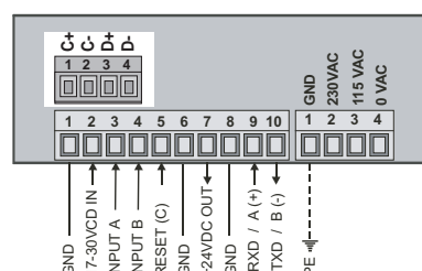
Display with serial interface 0.570.012.E05
