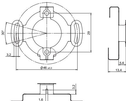
8.0010.4C00.0000 Double-winged stator coupling
